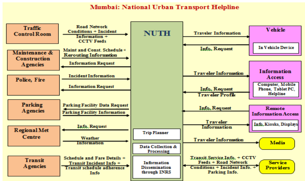
Figure 4-12: Mumbai NUTH Project Architecture
