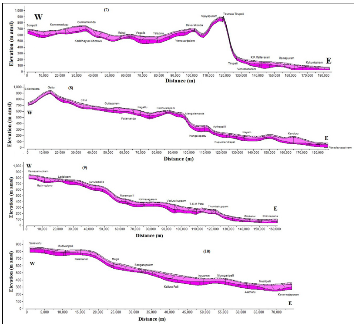
Fig-3.4 (7 to 10): West-east Sections, Chittoor district.
